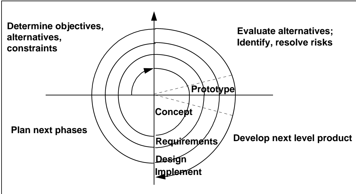
Figure 2 : Spiral Methodology
